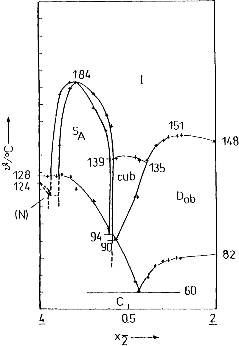
FIGURE 4 The isobaric phase diagram of the binary system of components 4/2
