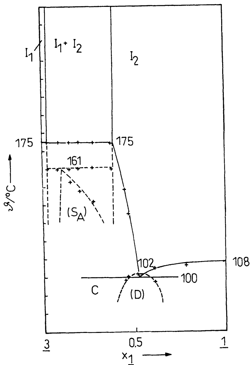
FIGURE 1 The isobaric phase diagram of the binary system of components \underline{3}/\underline{1} ( x = molar fraction); dotted lines correspond to transitions in the supercooled state
