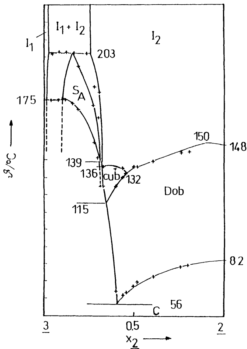
FIGURE 3 The isobaric phase diagram of the binary system of components 3/2
